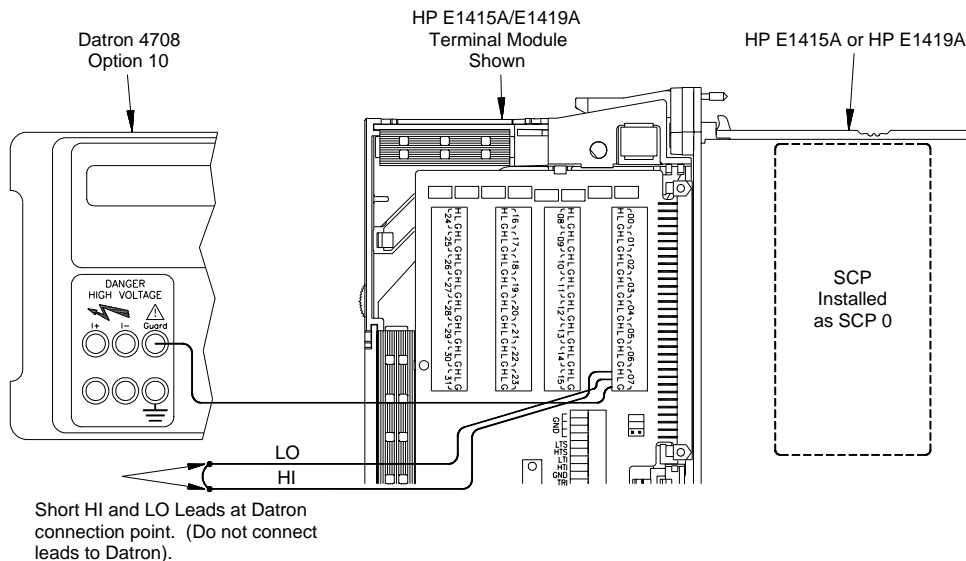
Figure 2-15. Channel Tare/Calibration Connections
