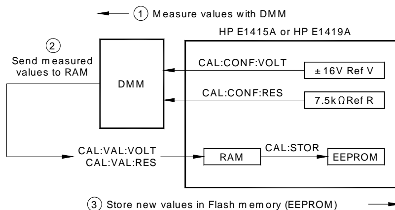
Figure 3-2. Adjustments
