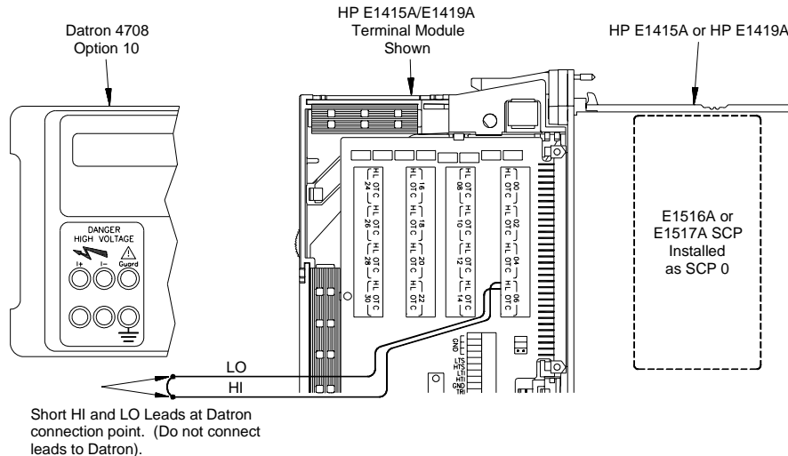
Figure 2-19. Channel Tare/Calibration Connections
