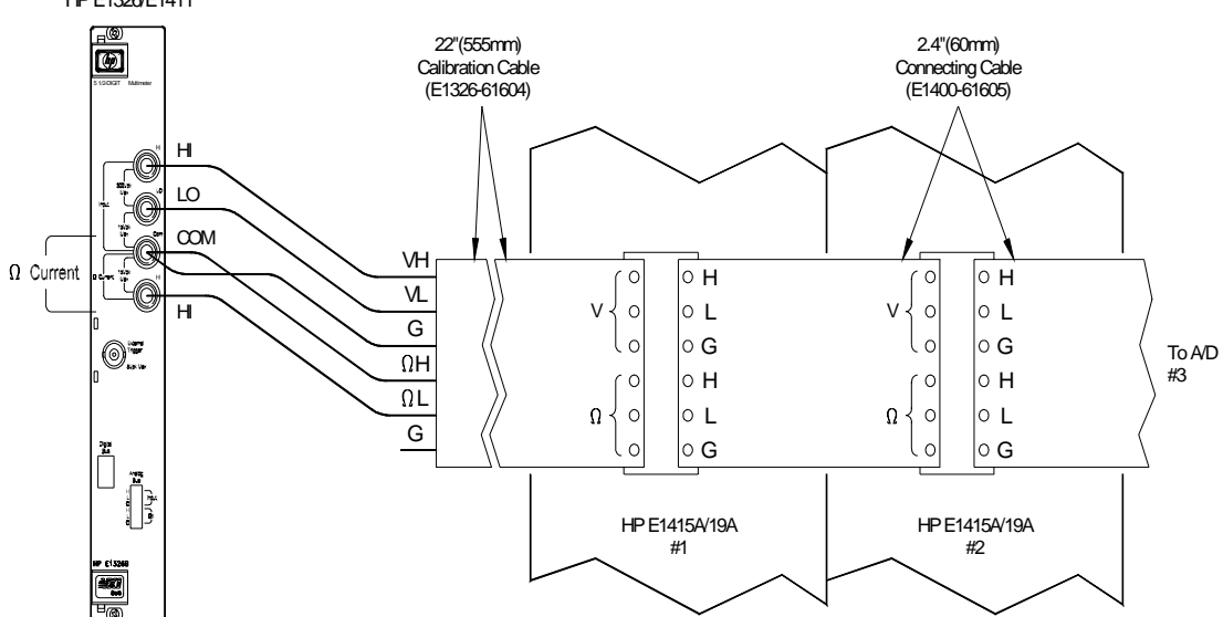
Figure 3-8. Cal Bus Connections
