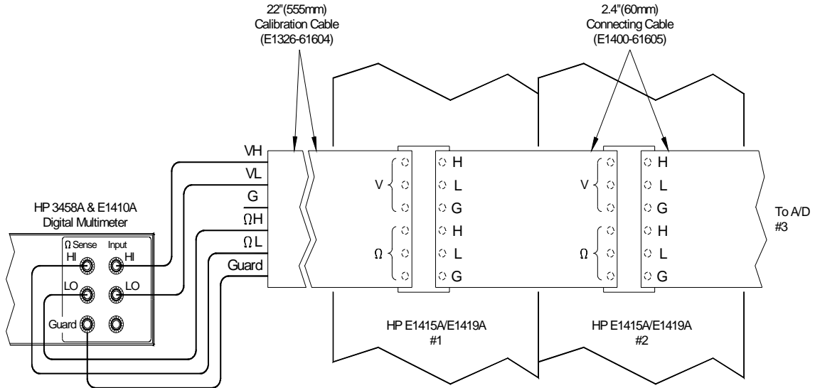
Figure 3-4. Cal Bus Connections
